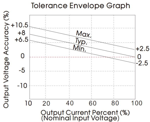
Fig. 1 Positive Output Voltage Tolerance Envelope Graph
