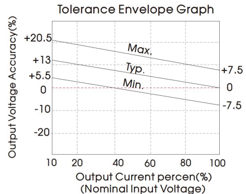
Fig. 2 Negative Output Voltage Tolerance Envelope Graph
