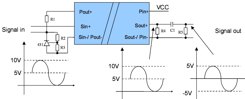
Fig. 3 Isolated transmission for electrical signals application
