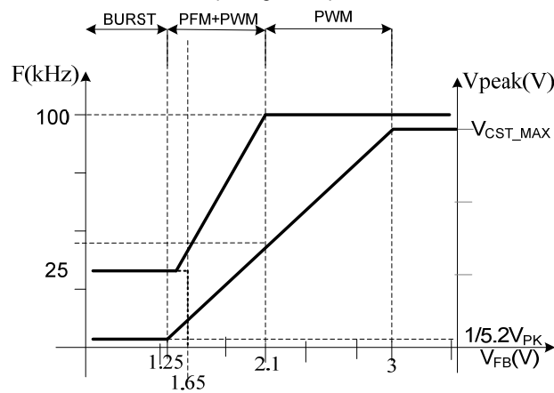
Fig.11 V_{FB} VS switching frequency and CS peak voltage
