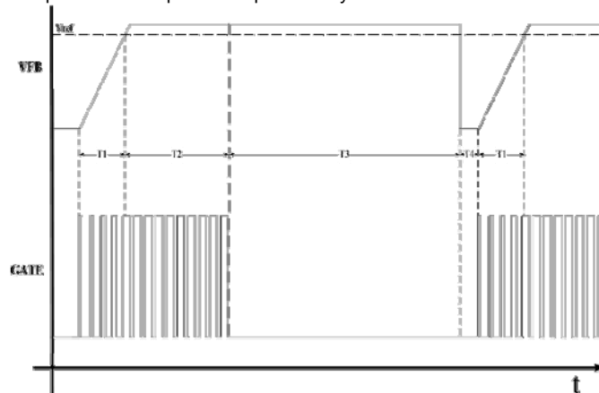
Fig.13 V_{FB} overvoltage protection sequence
