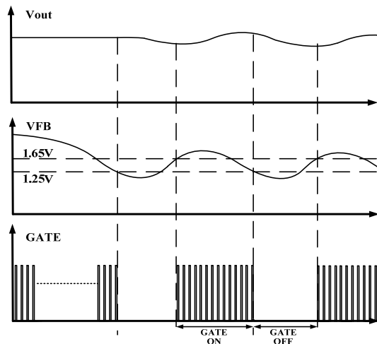
Fig.12 Burst mode time sequence
