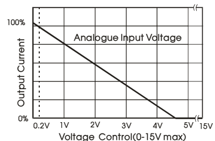
Fig. 9 Analogue input voltage and output current
