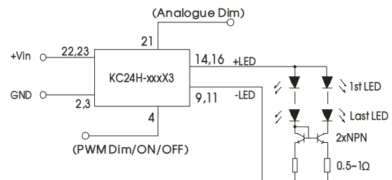
Fig. 3 Application circuits in series and parallel
