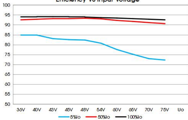
VCF4824EBO-100W(F)R3-N Efficiency VS Input Voltage
