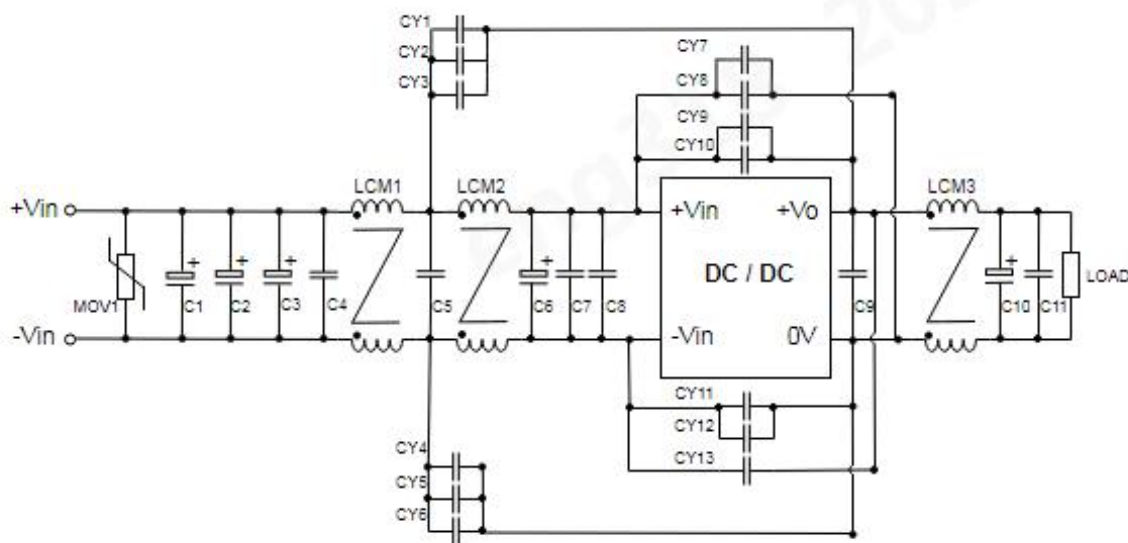
VCF4828/48EBO-100W(F)R3-N
