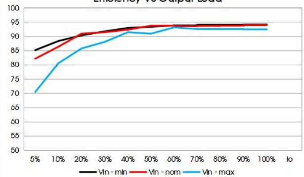
VCF4812EBO-100W(F)R3-N Efficiency VS Output Load
