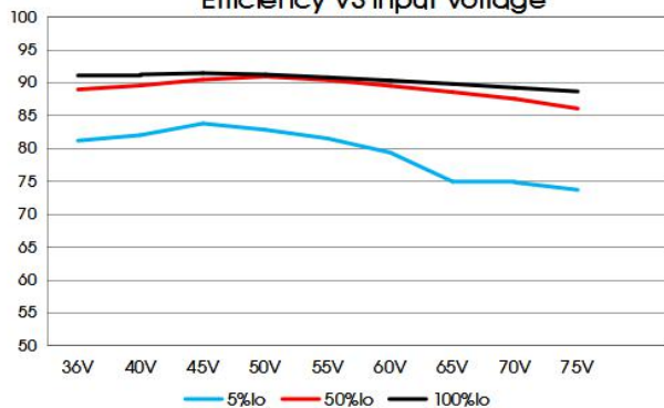
VCF4848EBO-100W(F)R3-N Efficiency VS Input Voltage
