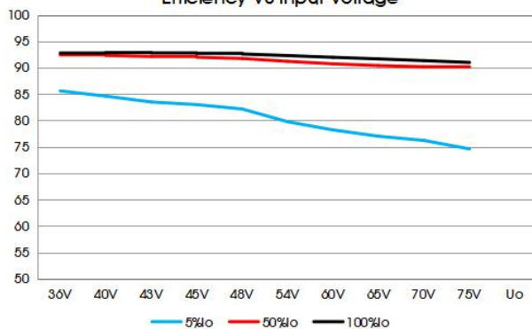
VCF4828EBO-100W(F)R3-N Efficiency VS Input Voltage
