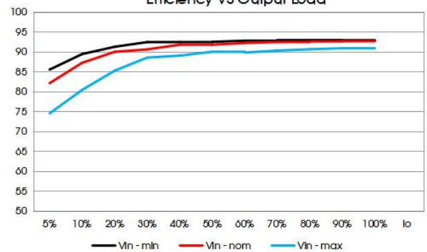
VCF4824EBO-100W(F)R3-N Efficiency VS Output Load
