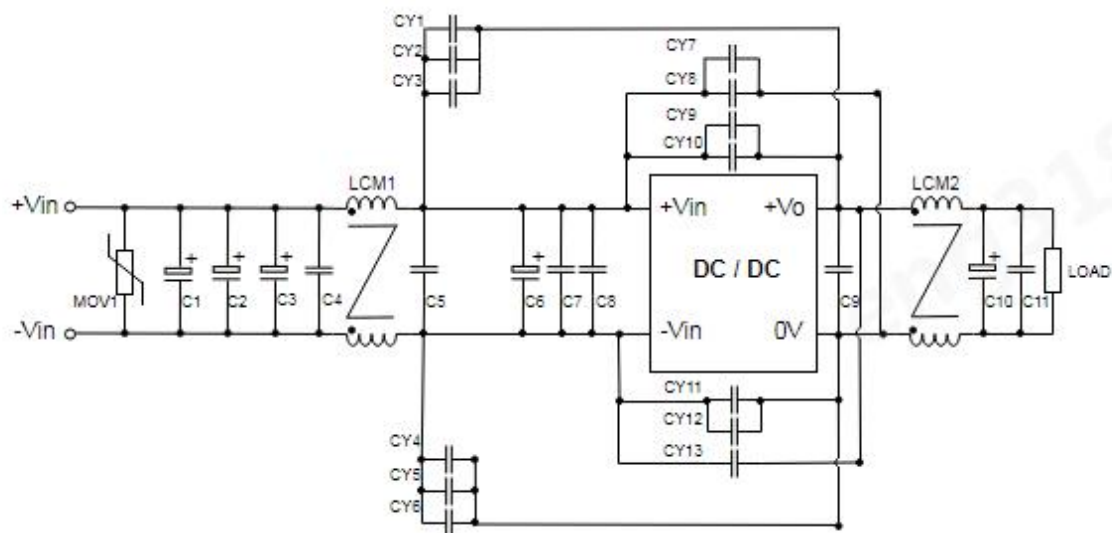
VCF4828/48EBO-100W(F)R3-N
