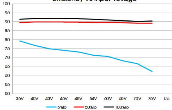
VCF4848EBO-100W(F)R3-N Efficiency VS Input Voltage
