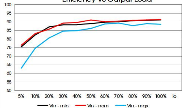
VCF4848EBO-100W(F)R3-N Efficiency VS Output Load
