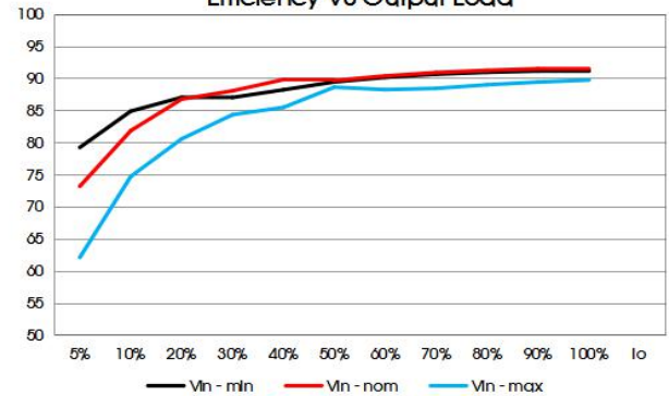
VCF4828EBO-100W(F)R3-N Efficiency VS Output Load
