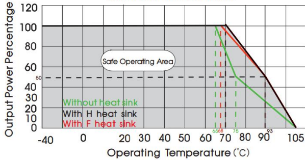
UWTH1D03/05/12/15LD-20W(H/F)R3 Temperature Derating Curve (Vin=110V, Without wind)
