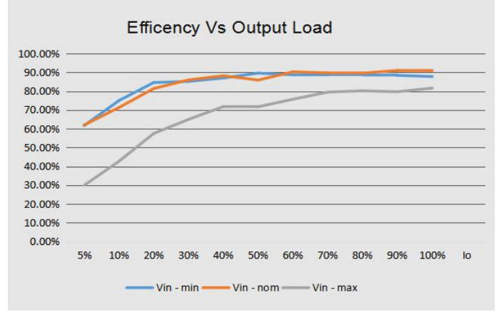
UWTH1D54LD-20WR3 Efficiency curve of output load (normal temperature)
