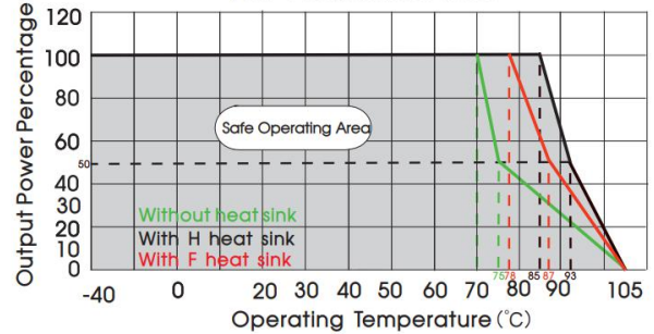
UWTH1D24/28/48/54LD-20W(H/F)R3 Temperature Derating Curve (Vin=110V, Without wind)
