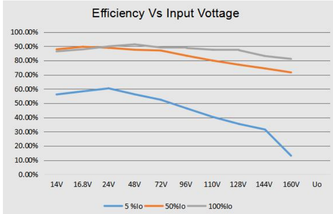
UWTH1D54LD-20WR3 Efficiency curve of input voltage (normal temperature)
