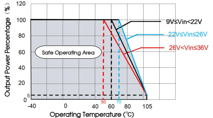
URB2424/28YMD-40WR3 Temperature Derating Curve
