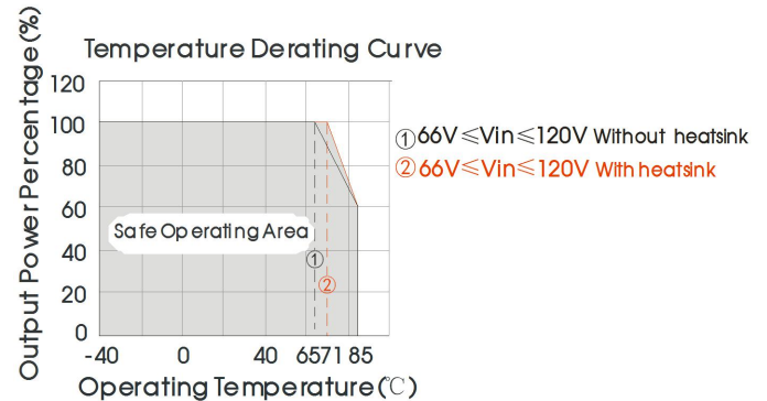
URB1D05LMD-20W(H)R3(A2S/A4S) Operating Temperature
