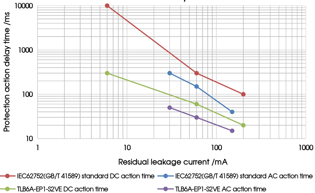
TLB6A-EP1-S2VE Module performance
