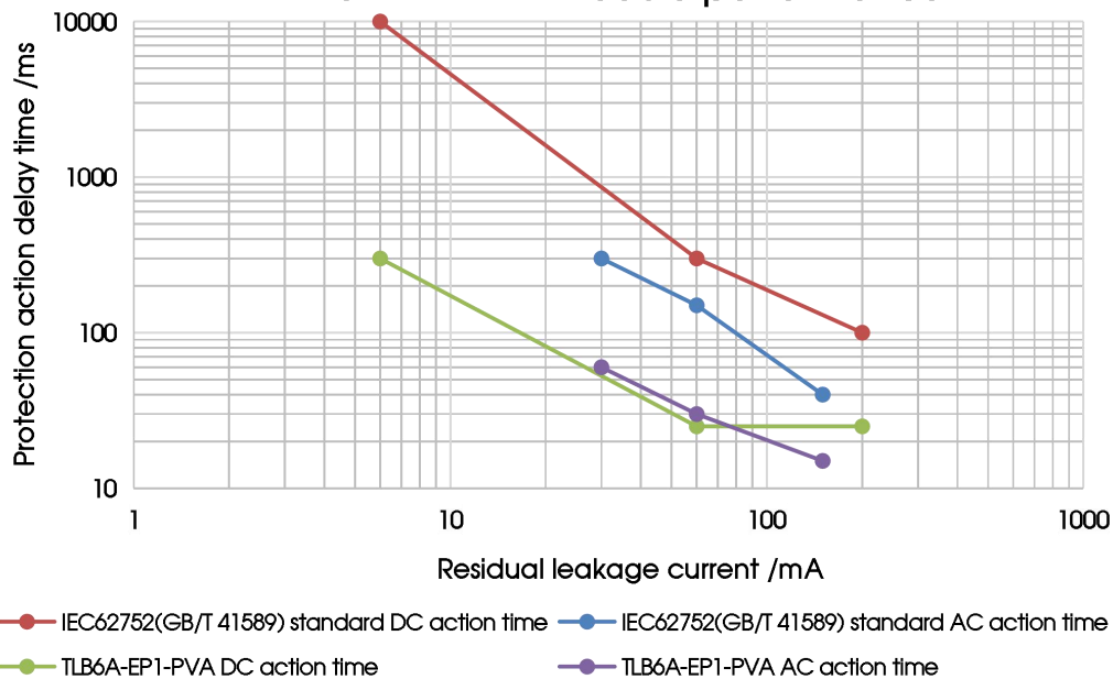
TLB6A-EP1-PVA Module performance
