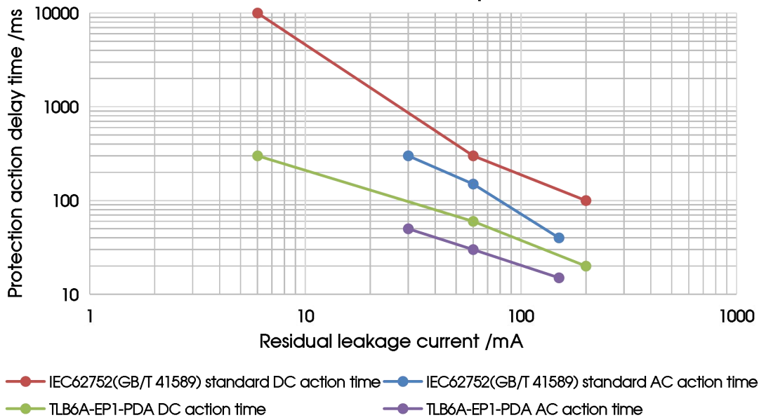
TLB6A-EP1-PDA Module performance
