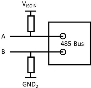
Figure13. Pull up and drop down resistance connect
