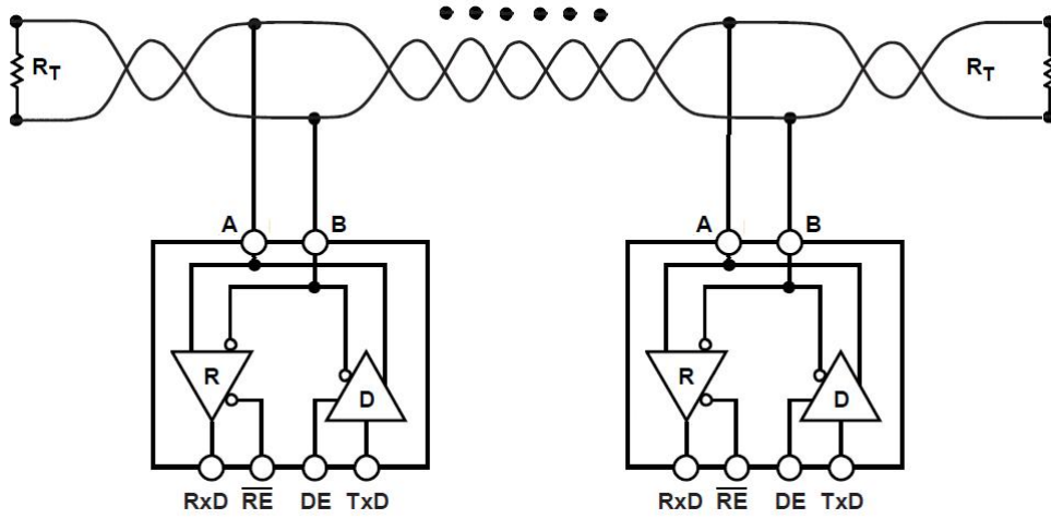
Figure10. Typical Application Circuit (Half-Duplex Network Topology)
