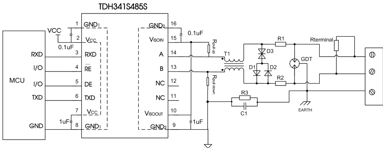
Figure12. Port protection circuit for harsh environments
