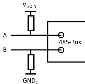
Figure13. Pull up and drop down resistance connect
