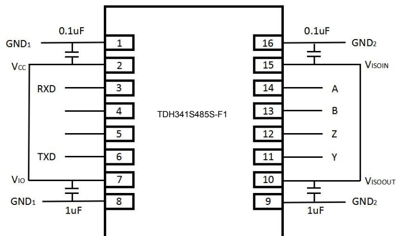
Fig 11. Typical Application of PCB layout
