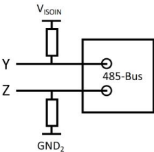
Fig 13. Typical connection of pull-up and pull-down resistors
