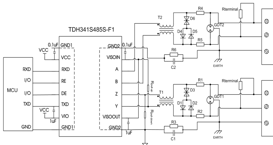
Fig 12. Port Protection Recommended Circuit
