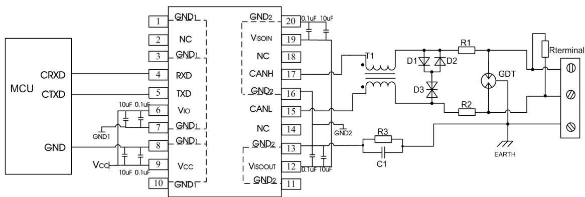
Figure26. Port protection circuit for harsh environments
