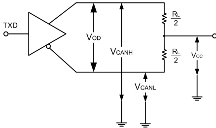
Figure 18. Driver test circuit
