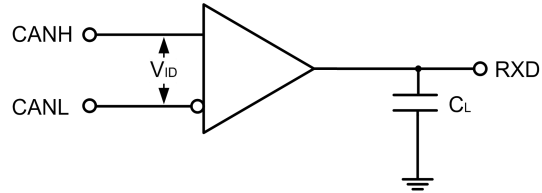
Figure 19. Receiver test circuit
