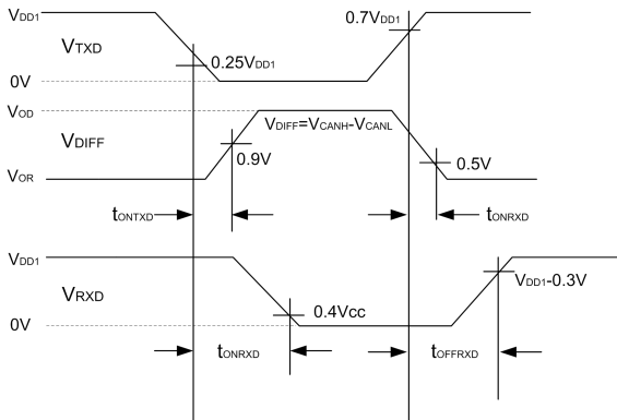
Figure 22. Drive and receiver propagation delay
