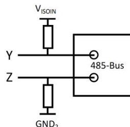
Figure14. Typical connection of pull-up and pull-down resistors
