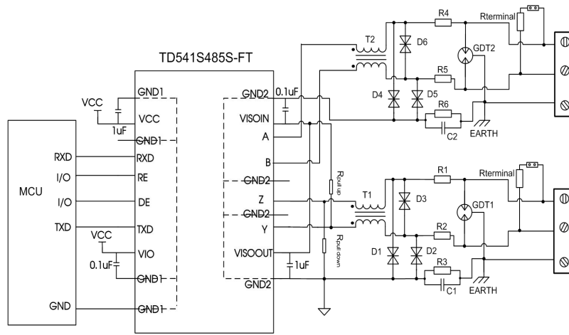
Figure13. Port Protection Recommended Circuit
