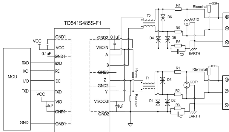
Figure12. Port protection circuit for harsh environments
