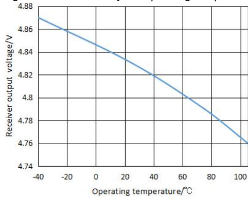
Figure 5. Receiver output high voltage vs. Operating Temperature
