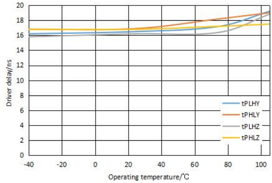
Figure 2. Driver delay vs. Operating Temperature
