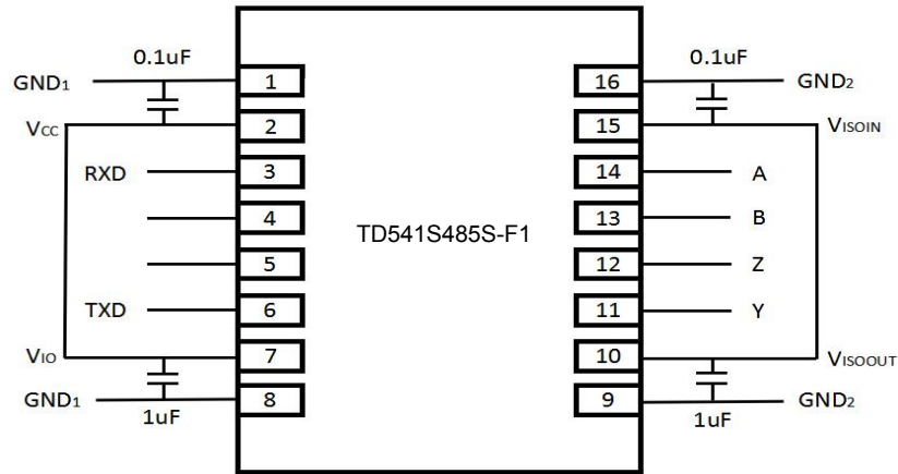
Figure11. Type PCB layout
