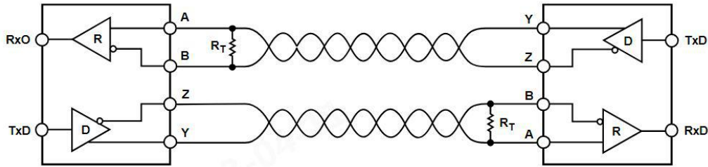
Figure10. Typical application circuit ( half-duplex network topology )
