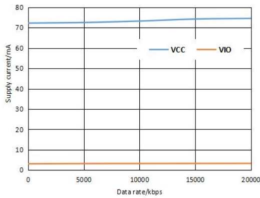
Figure 1. Supply current vs. Data rate
