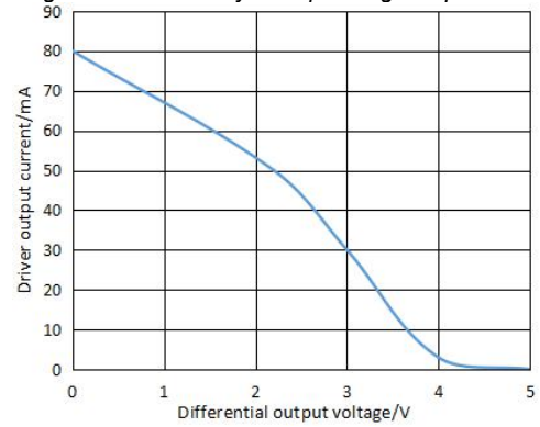
Figure 4. Driver output current vs. Differential output voltage
