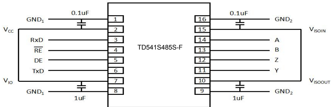
Figure12. Type PCB layout
