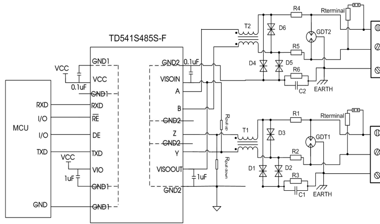
Figure13. Port protection circuit for harsh environments
