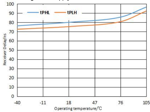
Figure 3. Receiver delay vs. Operating Temperature
