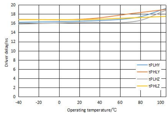
Figure 2. Driver delay vs. Operating Temperature
