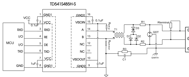
Figure12. Port protection circuit for harsh environments
