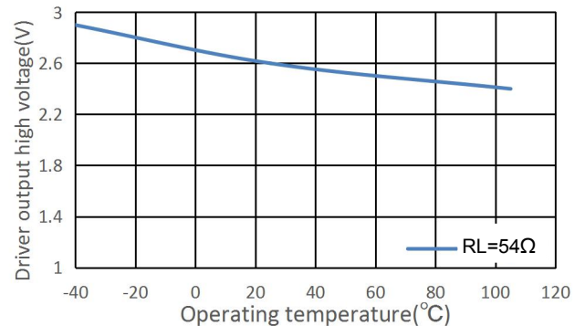
Figure 4. Driver output high voltage vs. Operating Temperature
