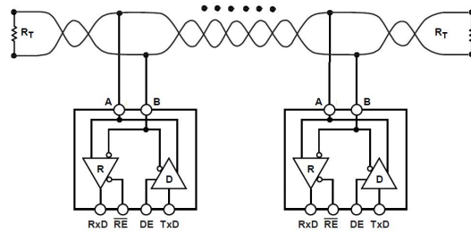
Figure10. Typical application circuit (half-duplex network topology) VISIO
