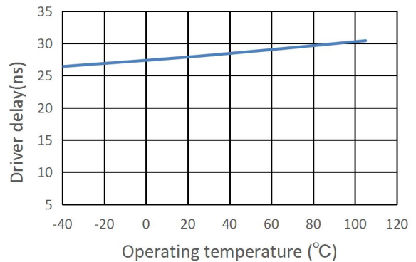
Figure 2. Driver delay vs. Operating Temperature
