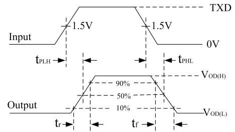
Figure 7. Drive propagation delay test circuit and wave forms
