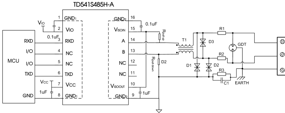
Figure10. Port protection circuit for harsh environments
