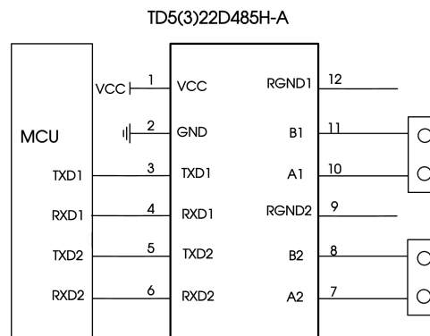
Fig.1: Typical application
