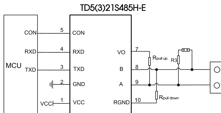
Fig. 1: Typical application
