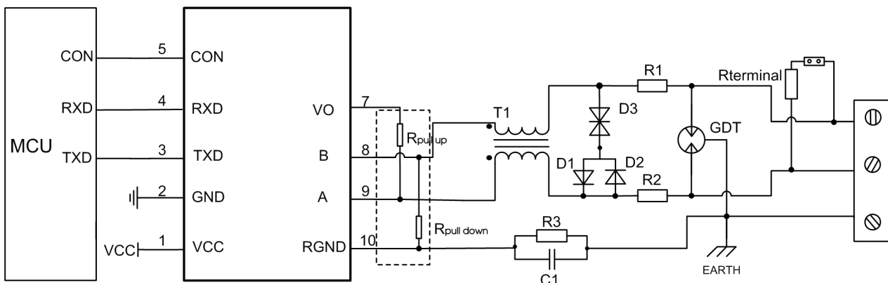
Fig. 2: Port protection circuit for harsh environments
