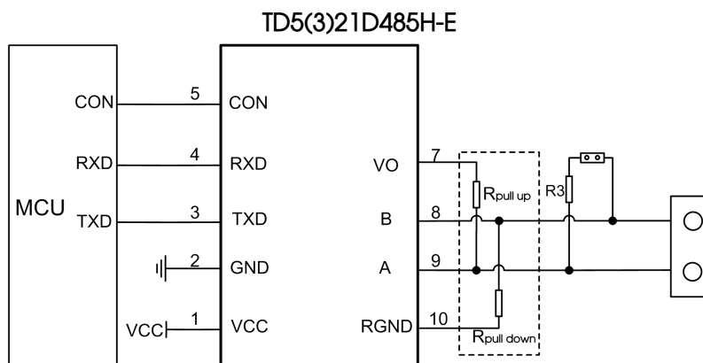
Fig. 1: Typical application
