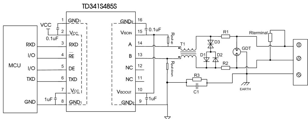
Figure12. Port protection circuit for harsh environments
