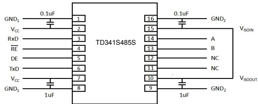
Figure11. Typical Application of PCB layout
