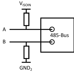
Figure13. Pull up and drop down resistance connect
