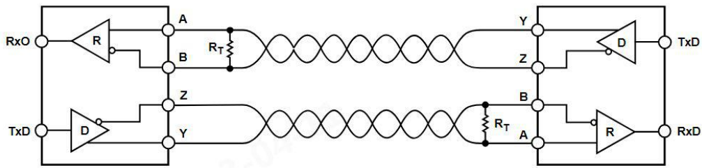
Fig 10. Typical Application Circuit (Full-Duplex Network Topology)
