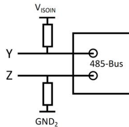
Fig 13. Typical connection of pull-up and pull-down resistors
