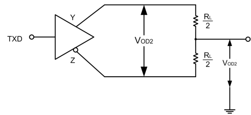
Fig 7. Differential output test circuit
