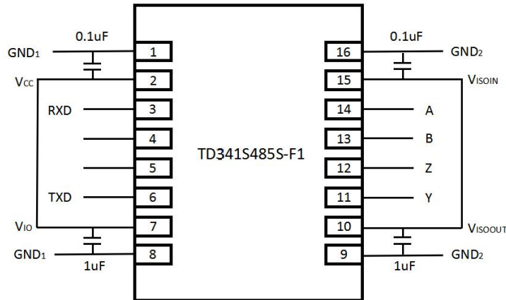
Fig 11. Typical Application of PCB layout
