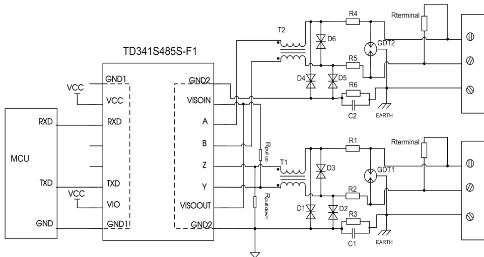
Fig 12. Port Protection Recommended Circuit
