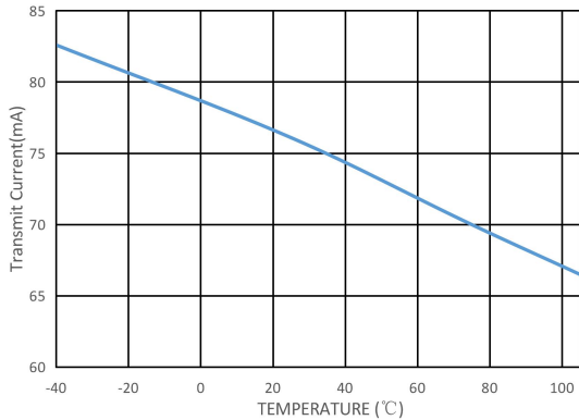
Figure4. Transmit Current vs. Temperature, V_{DD1}=5V , V_{DD2}=5V
