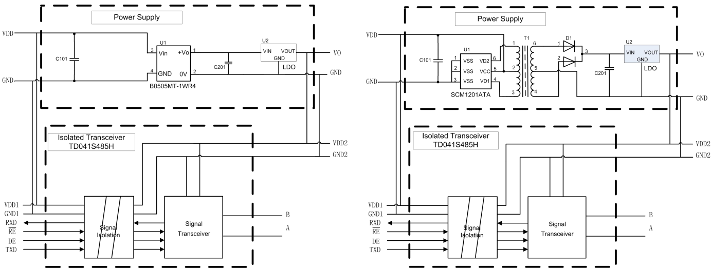
Figure 13. Receiver propagation delay test circuit and wave forms
