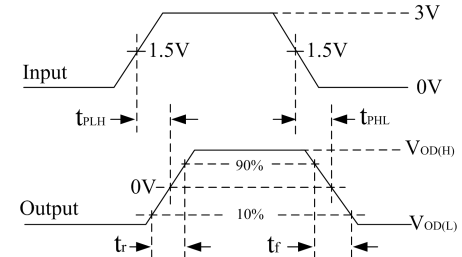
Figure 11. Drive propagation delay test circuit and wave forms
