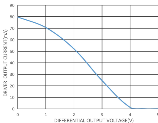
Figure 6. Driver Output Current vs. Differential Output Voltage
