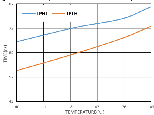
Figure 8. Receiver Propagation Delay vs. Temperature
