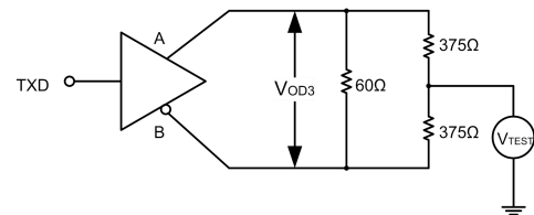
Figure 10. Driver Test Circuit, VOD With Common-Mode Loading
