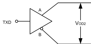
Figure 6. Driver Test Circuit
