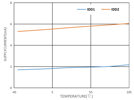
Figure2. Transmit Current vs. Temperature, VDD1=5V, VDD2=5V
