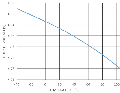
Figure3. Receiver Output High Voltage vs. Temperature, VDD1=5V, VDD2=5V
