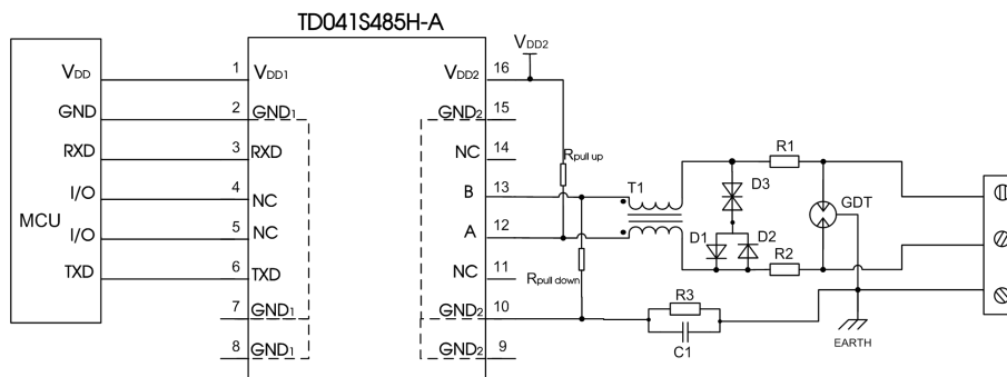
Figure 10. Port protection circuit for harsh environments
