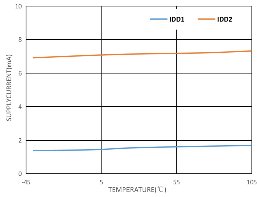
Figure1. Unloaded Supply Current vs. Temperature
