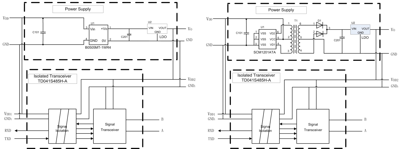
Figure 9. Typical application circuit
