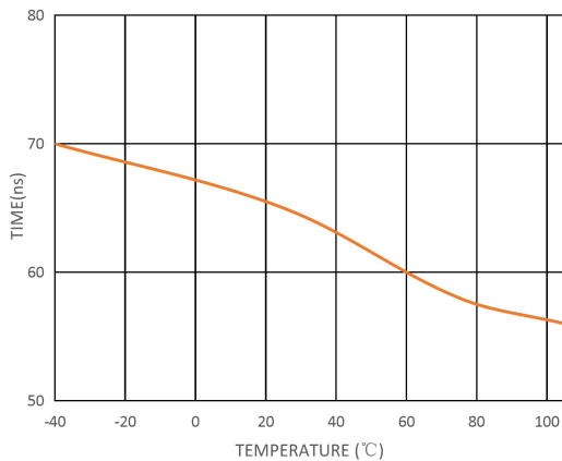
Figure 5. Receiver Propagation Delay vs. Temperature
