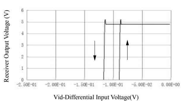
Figure 12 Receiver output voltage vs. Differential input voltage
