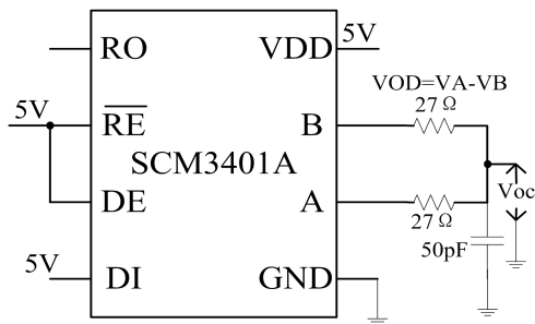
Figure 18 Driver V_{OC} Test Circuit
