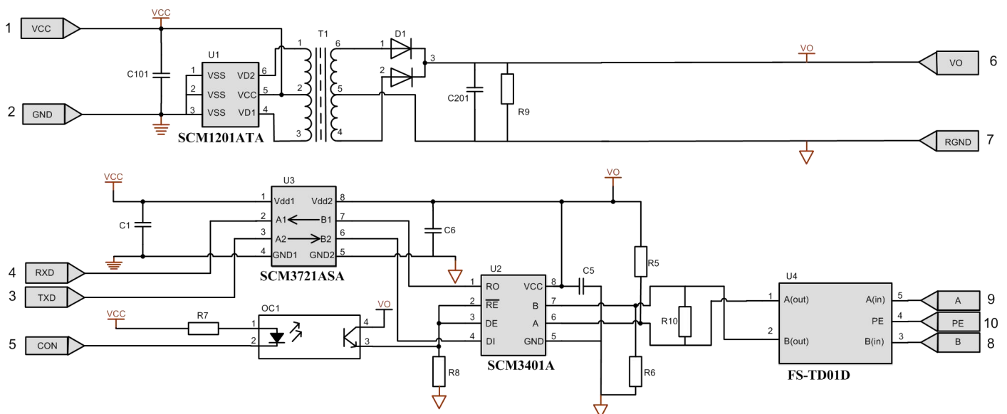
Fig. 26 Schematic diagram of isolation application circuit for UART to RS485 signal
