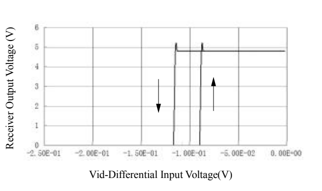
Figure 12 Receiver output voltage VS Differential input voltage
