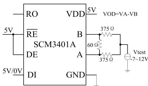
Figure 17 Driver Test Circuit, V_{OD} With Common-Mode Loading
