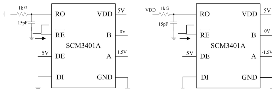
Figure 24 Receiver Enable/Disable Test Circuit and Waveforms, Data Output Low
