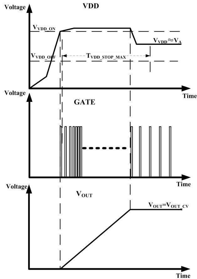
Fig. 16: Startup timing
