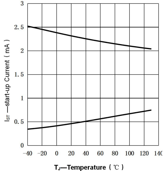
Fig. 2 Start-up Current vs. Temperature
