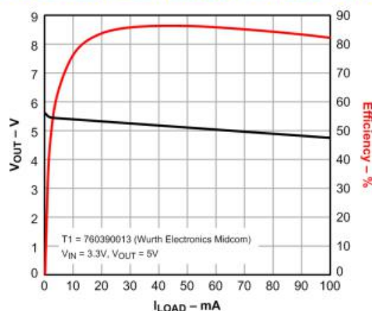
Output Voltage and Efficiency vs Output Current
