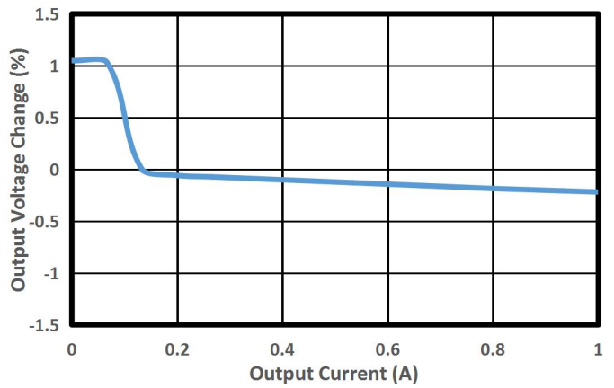
Figure 4. Load Regulation ( V OUT =12V, L=47μH)
