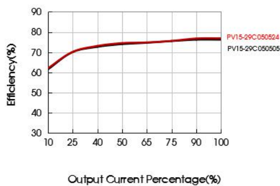
Efficiency Vs Output Load (Vin=600VDC)
