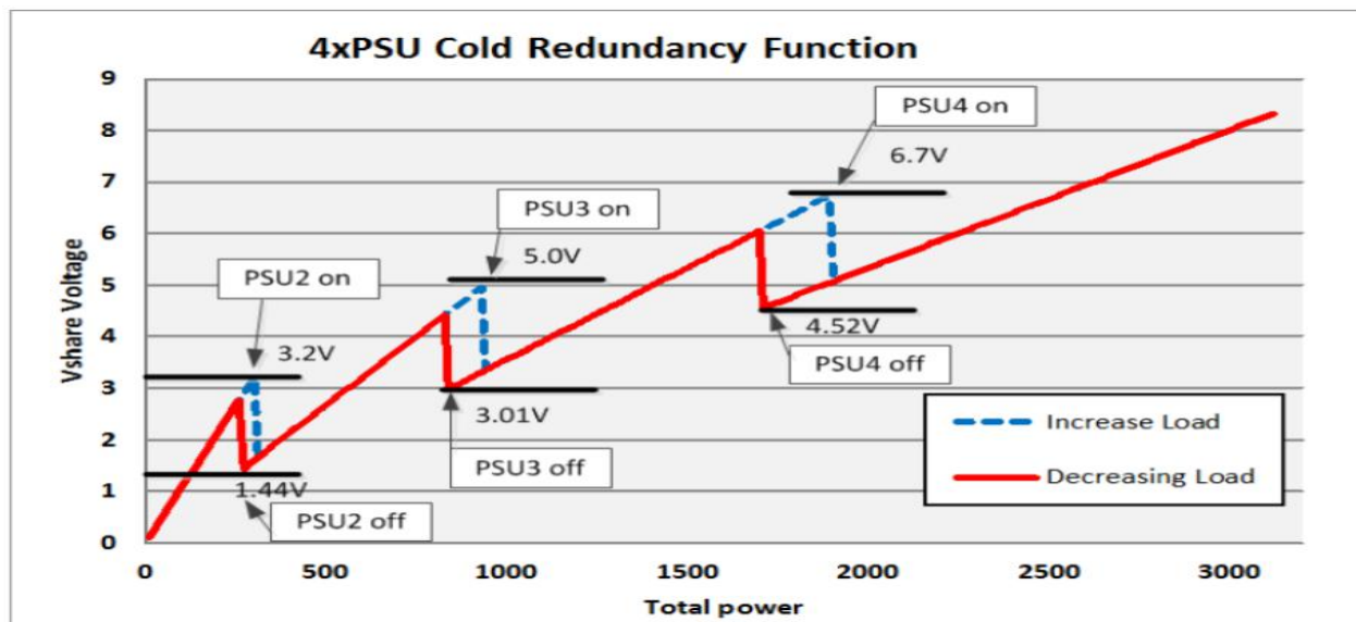
Power on/off in cold redundancy mode (4x PSUs)
