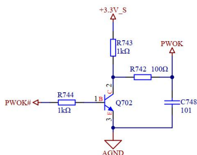
PWOK Signal Characteristics
