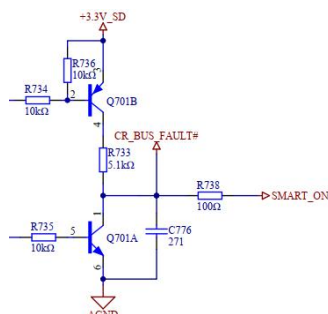
SMART_ON Signal Characteristics
