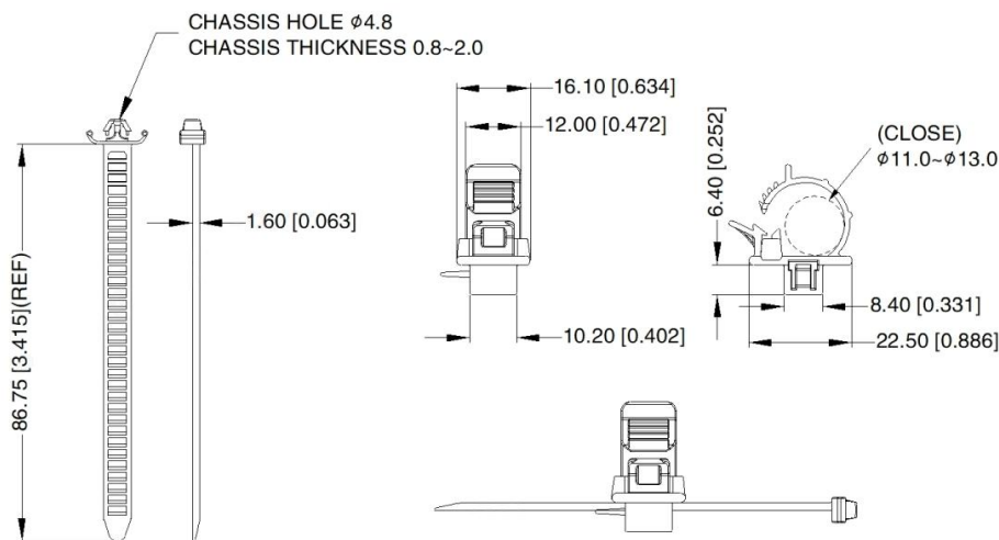
Assembly Drawing
