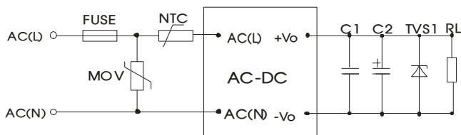
Fig. 1: LH40-10Bxx typical application circuit
