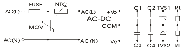
Fig. 2: LH40-10Axx typical application circuit
