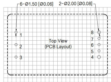
Pin-Out
