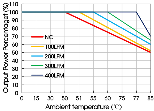
Temperature Derating Curves (Vo=1.0V)
