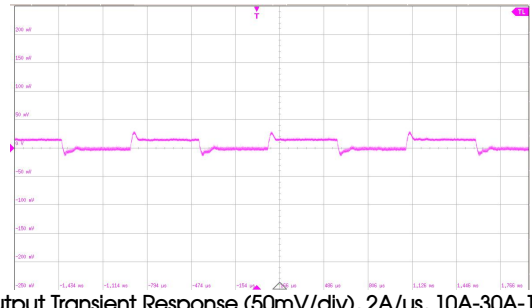
Output Transient Response (50mV/div), 2A/us, 10A-30A-10A, Bandwidth: 20MHz
