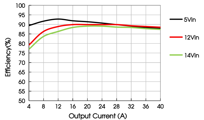
Efficiency Vs Output Load(Vout=1.0V)
