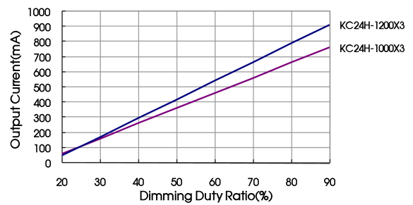
Fig. 8 Dimming duty ratio and output current (f=200Hz)
