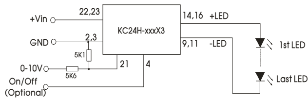
Fig. 9 Analogue dimming circuit
