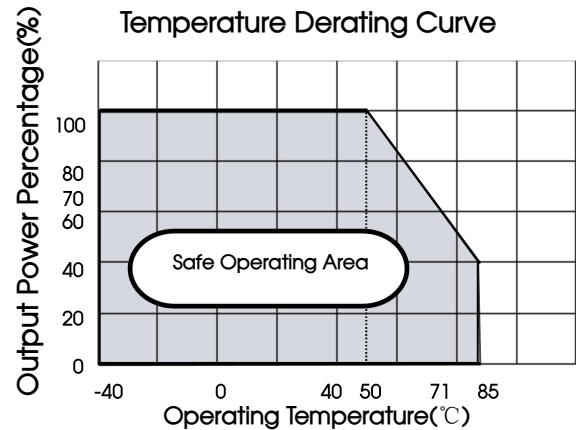
Fig. 1-③ Free air convection curve (Negative output)
