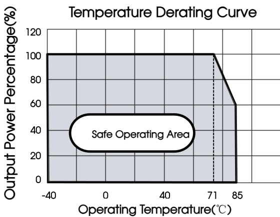
Fig. 1-③ Free air convection curve (Negative output)
