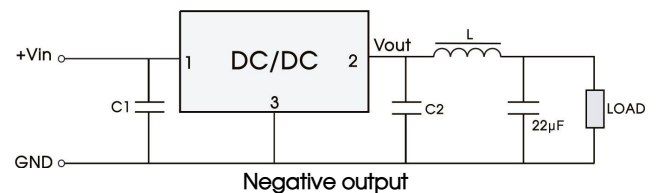
Fig. 4 External "LC" output filter circuit diagram
