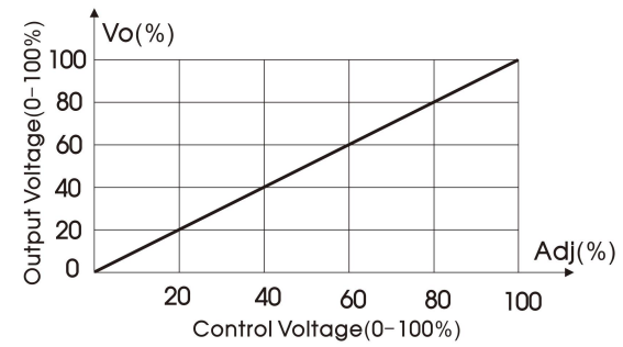
(Note: 100% Adj is equal to 5.0VDC (Typ.)) The relationship curve of output voltage and control voltage
