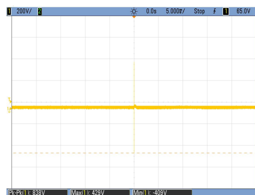
Output voltage waveform (0.42 KV)
