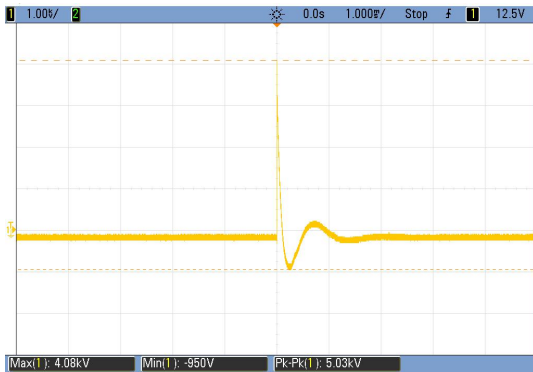
Input voltage waveform (Common mode 4.08kV)
