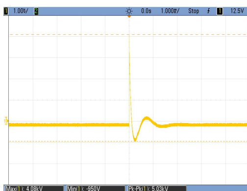
Input voltage waveform (Common mode 4.08KV)
