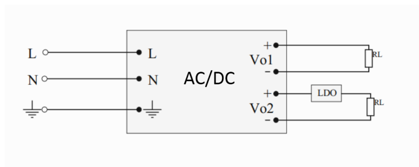
Figure 3-4 Typical application diagram of dual output
