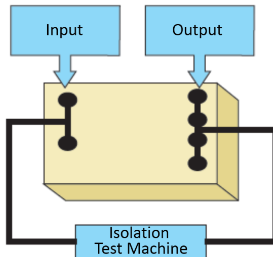
Figure 4-3 Isolation Test
