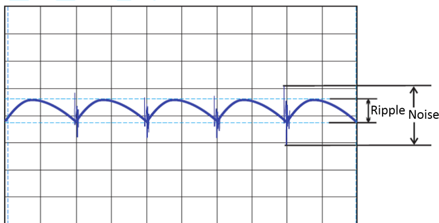
Figure 4-2 Waveform of Ripple and Noise Test
