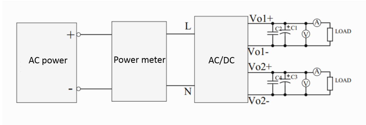
Figure 3-2 Multi-output basic test circuit connection
