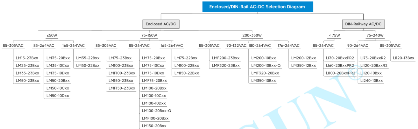
Figure 2-1 Enclosed/DIN-Rail AC/DC Selection Diagram
