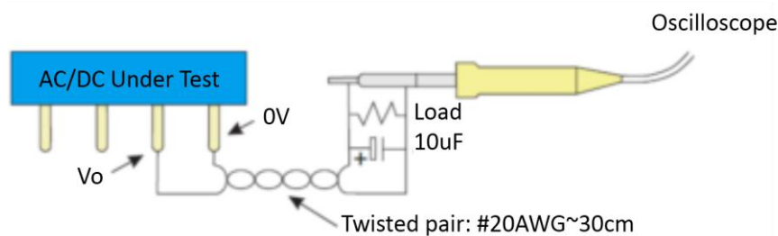
Figure 4-1 Twisted pair test method
